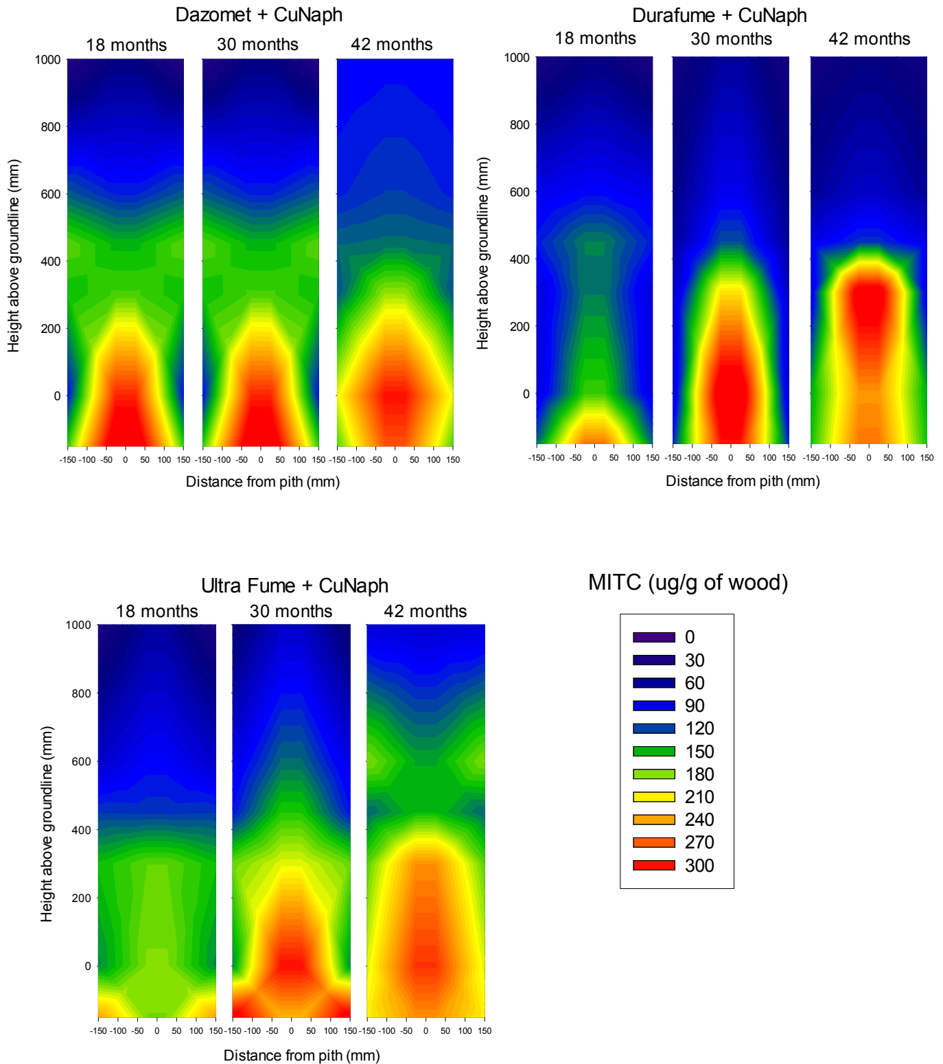
Figure I-12. Distribution of MITC in Douglas-fir poles sections 18 to 42 months after treatment with dazomet plus copper naphthenate, DuraFume plus copper naphthenate or UltraFume plus copper naphthenate.
